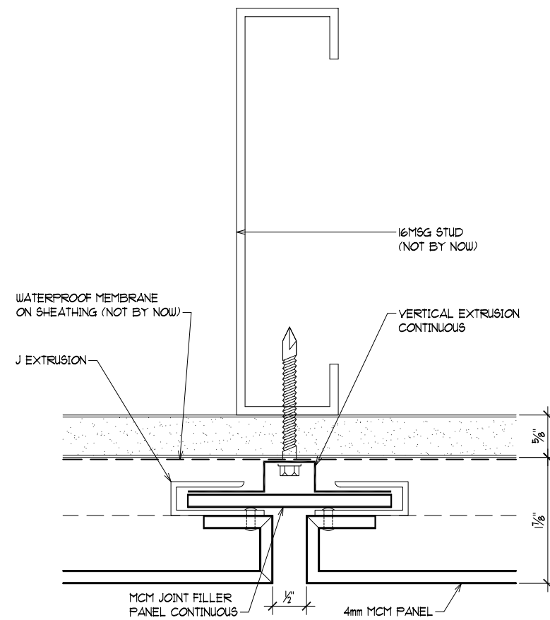
610 DJ VERTICAL JOINT DETAIL SCALE: HALF SCALE REF. ARCH:
