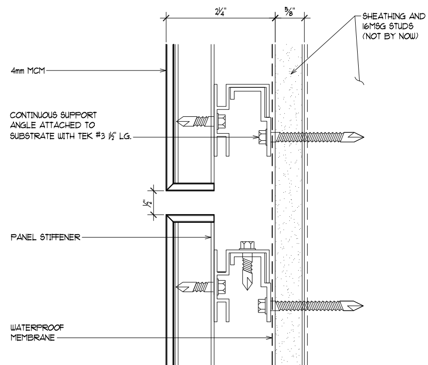
HORIZONTAL JOINT DETAIL
