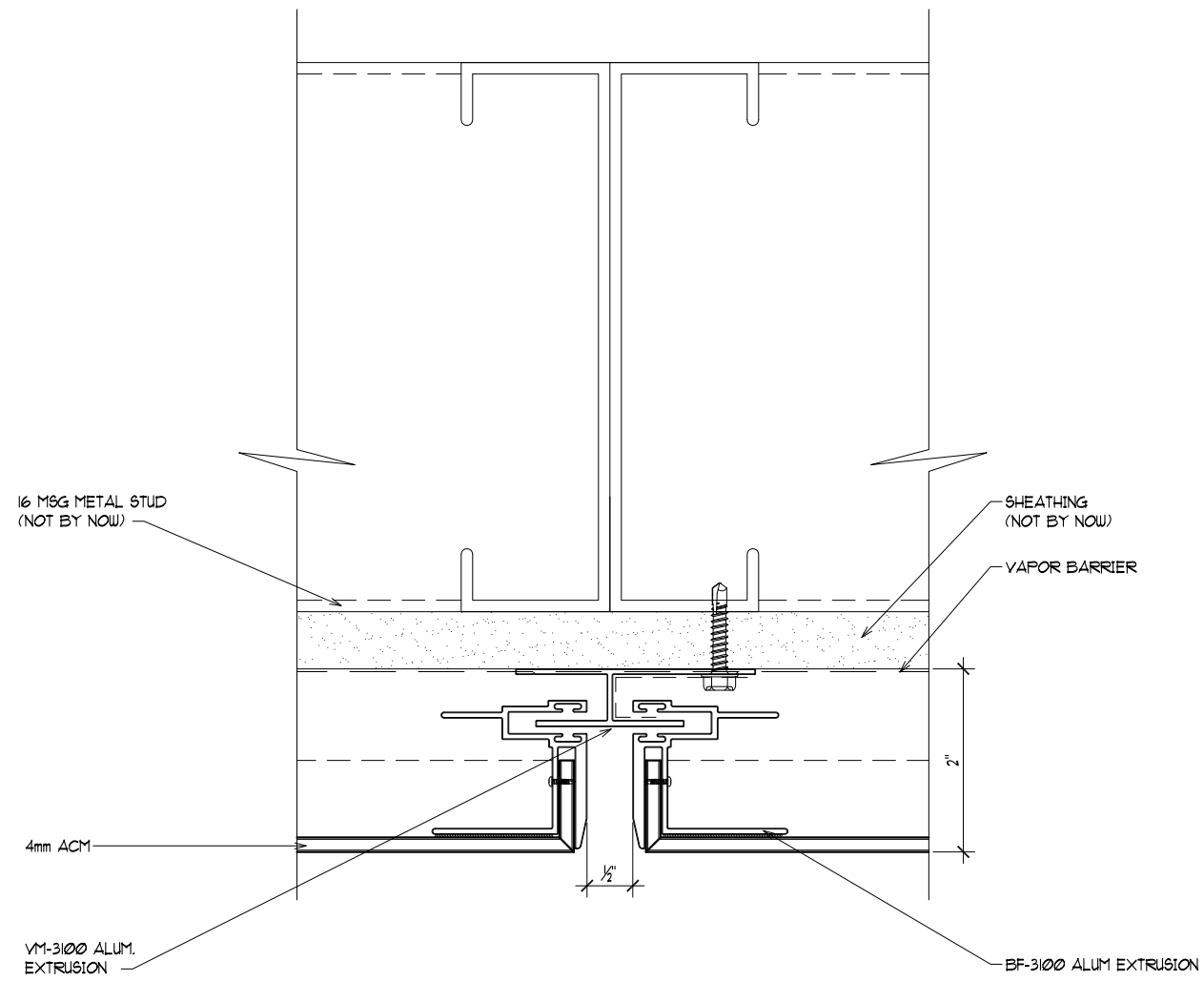
VERTICAL JOINT DETAIL
