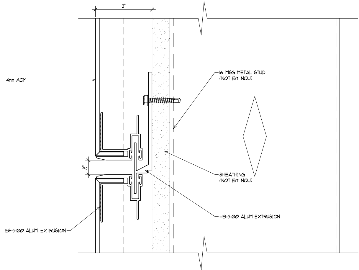
HORIZONTAL JOINT DETAIL
