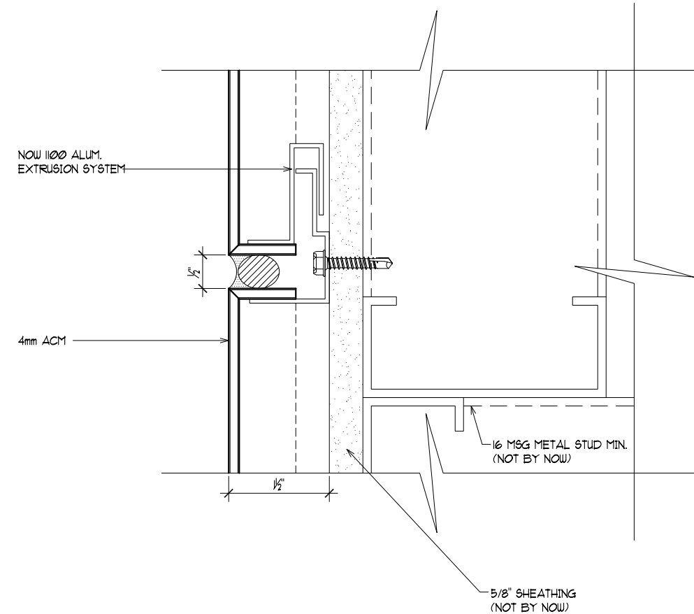
615 D1 HORIZONTAL JOINT DETAIL SCALE: HALF SCALE REF. ARCH:
